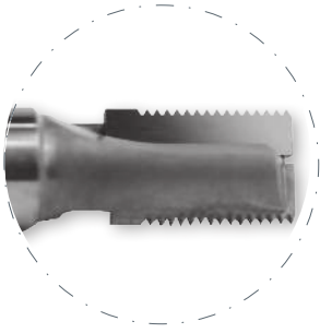
Profiled cutters
