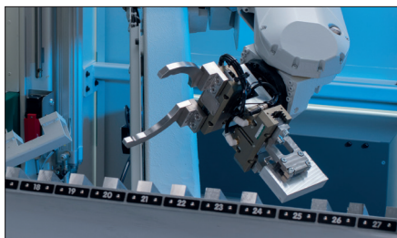
Articulated-arm robot: handling of pallets and blanks with a single system
